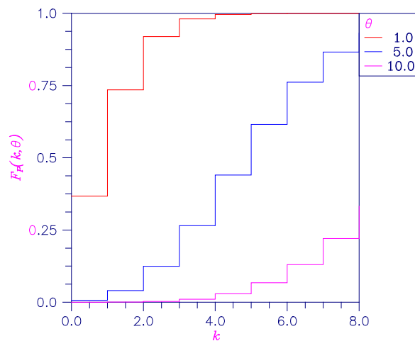
Figure 9-4 Plot of F_p(k, \theta)
