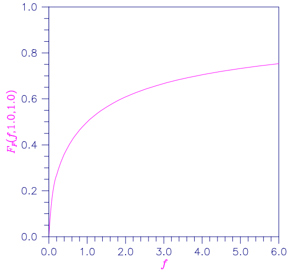
Figure 9-2 Plot of FF (f, 1.0, 1.0)
