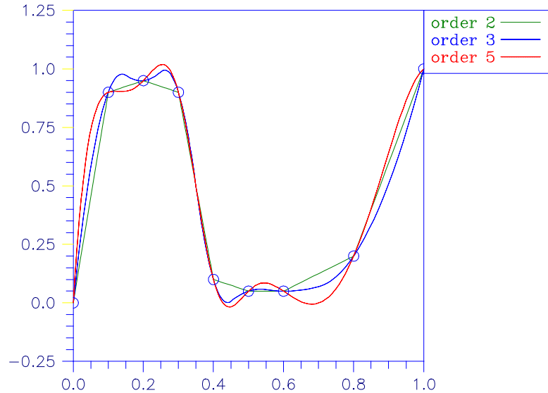
Figure 3-4 Three Spline Interpolants
