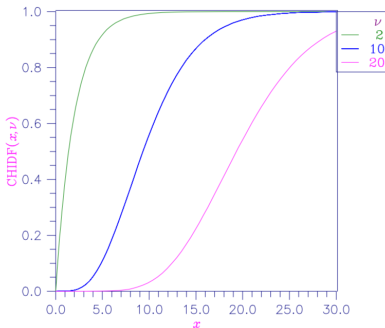
Figure 9-14 Plot of F_X(x, df)
