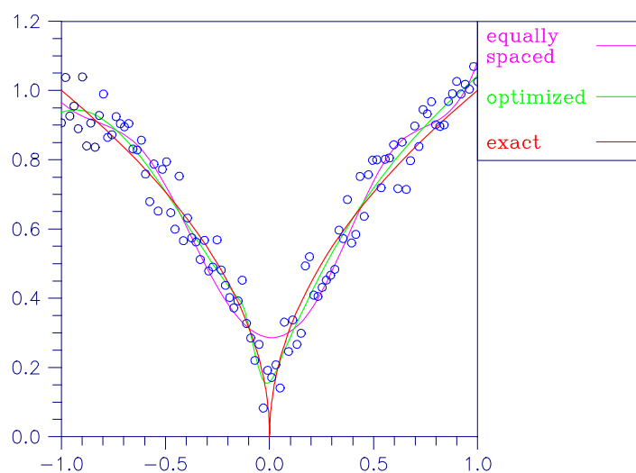
Figure 3-5 Two Fits to Noisy \sqrt{|x|}
