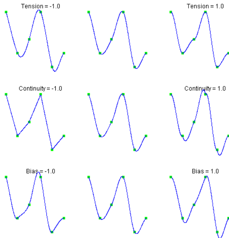
Figure 3-3 Data Points Interpolated with Different Parameter Values
