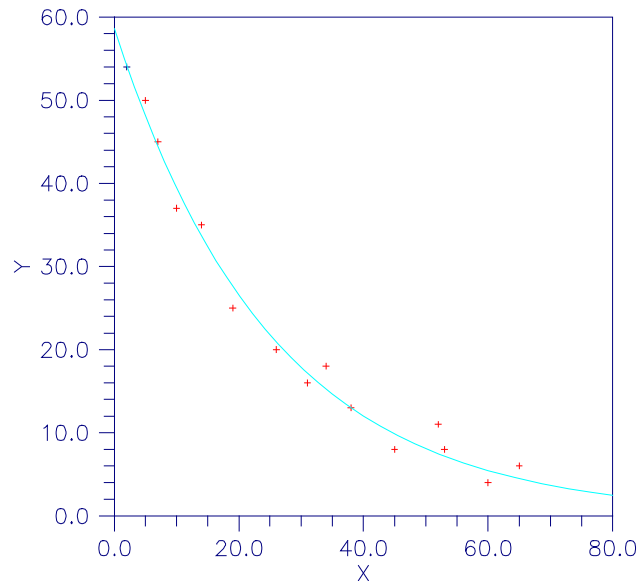
Figure 8-1 Plot of the Nonlinear Fit
