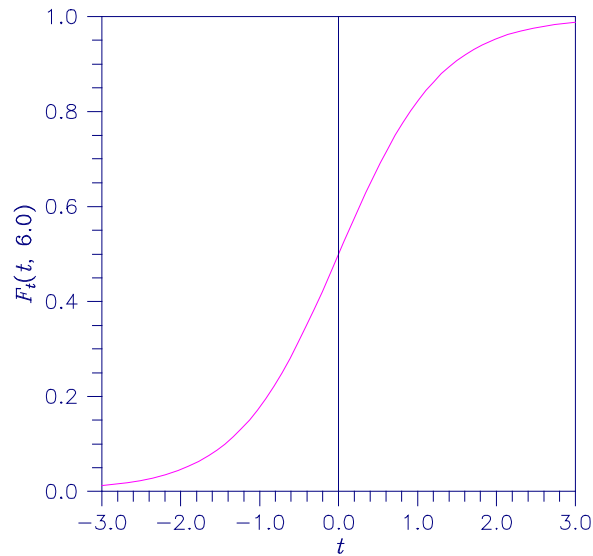
Figure 9-3 Plot of F_t(t, 6.0)
