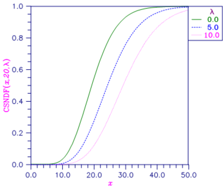
Figure 30, Noncentral Chi-squared Distribution Function
